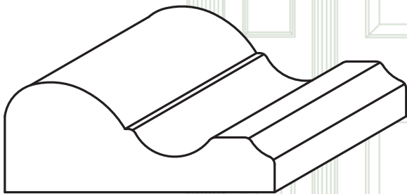
2664-P 1\frac{3}{16} " x 2" CHE, OAK, POP
